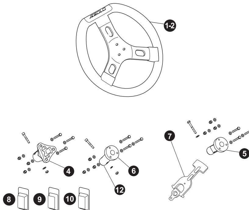
Piantone Sterzo Steering Collumn
